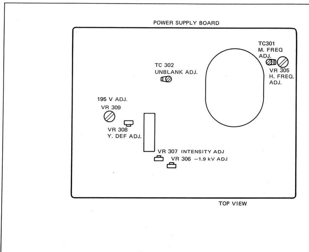
Fig. 8 Rear Printed Circuit Board (X68-1190-00)
