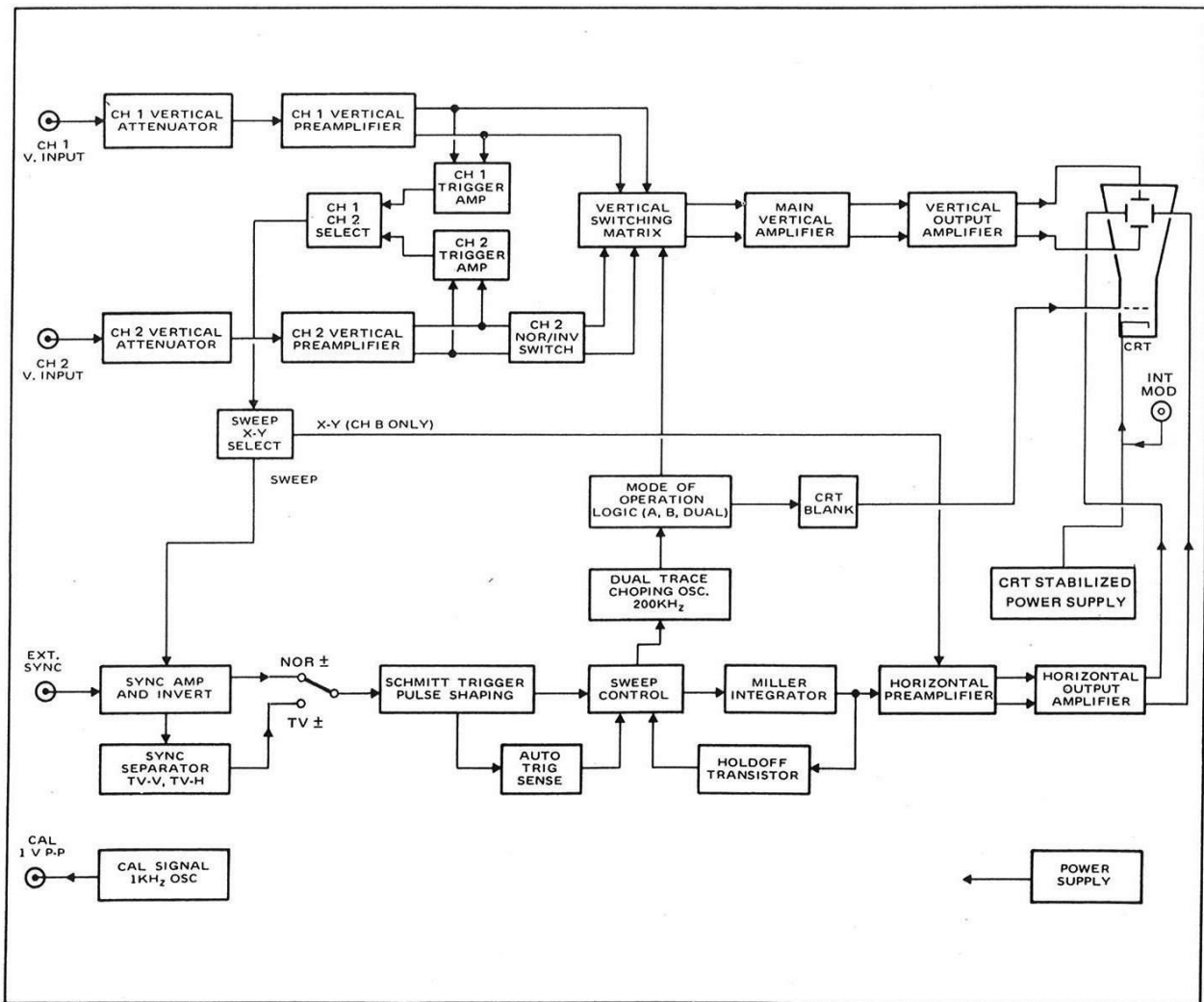
Fig. 1 Block Diagram, CS-1560A Dual-Trace Oscilloscope
