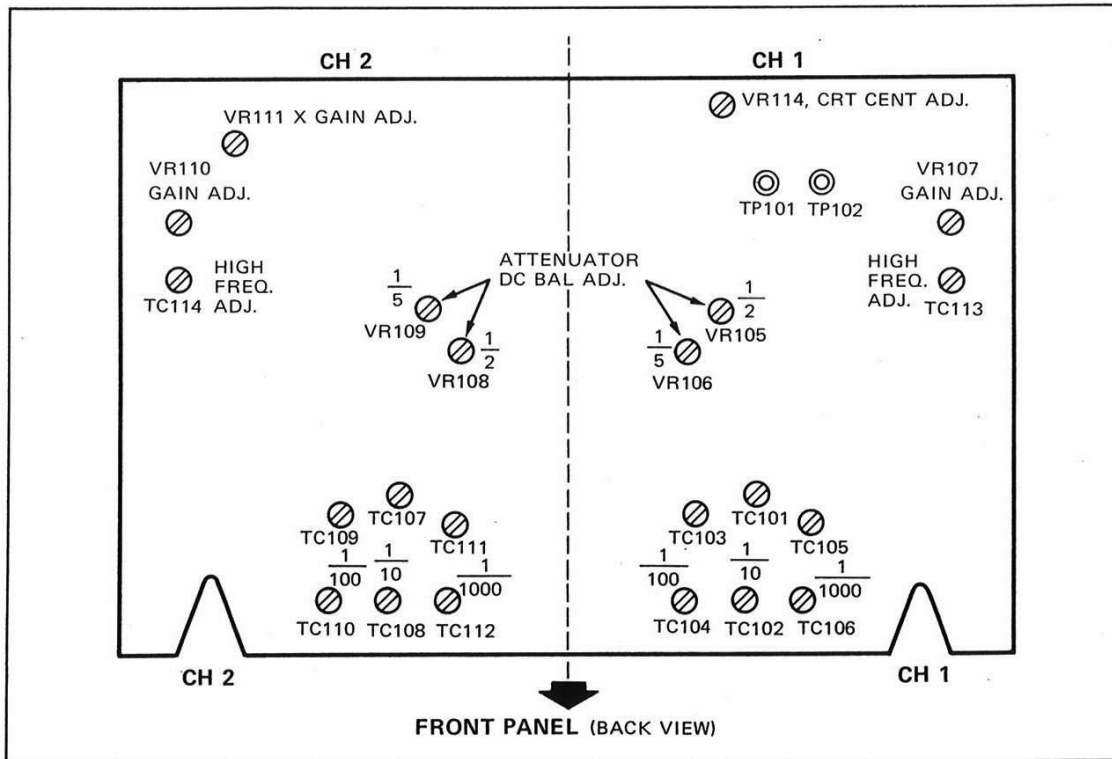
Fig. 7 Lower Printed Circuit Board (X73-1230-00)
